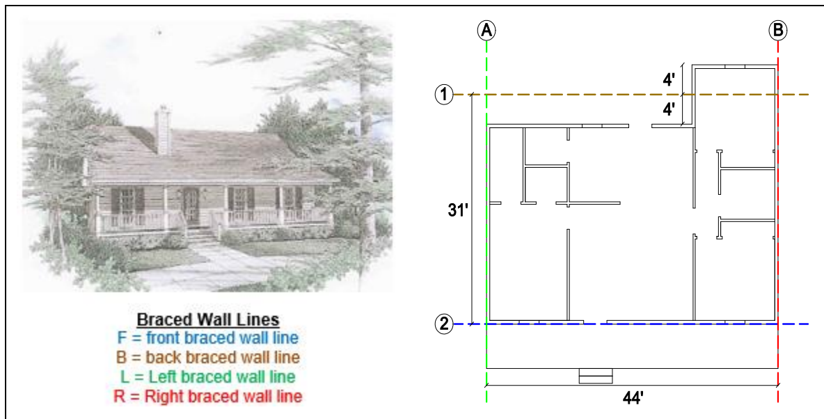
Figure 17. House Plan for Example #B1 with Designated Braced Wall Lines
