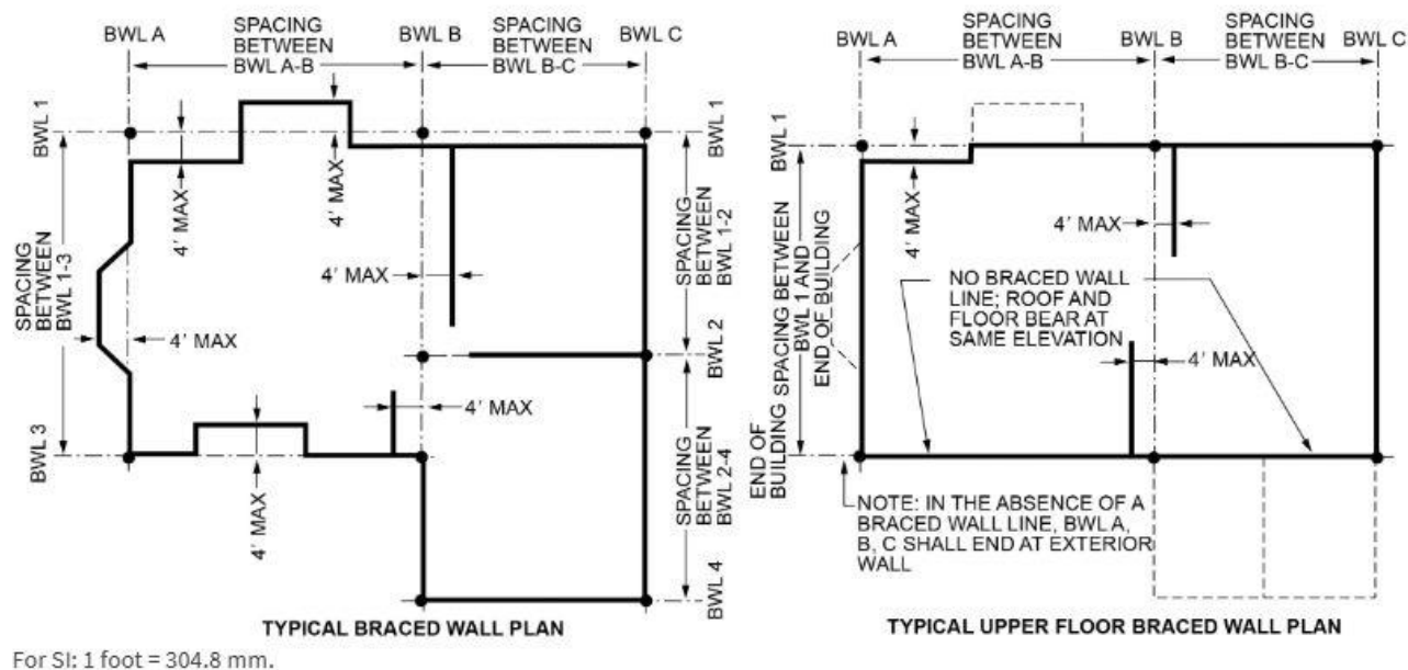
Figure 3. Braced Wall Lines – IRC Figure R602.10.1.1 6
