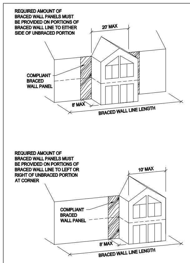
Figure 11. Limits for Large Openings in Braced Wall Lines with Intermittent Bracing
